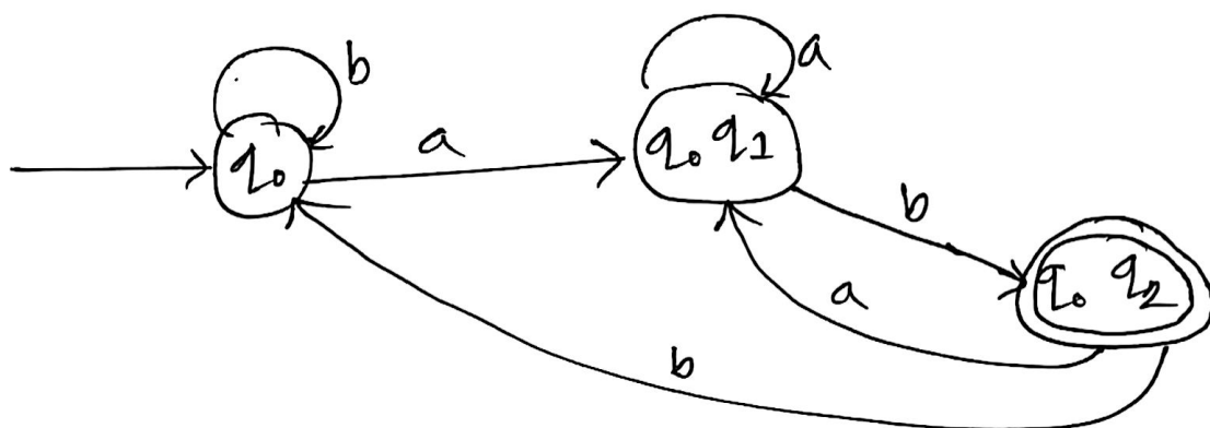
DFA diagram:
